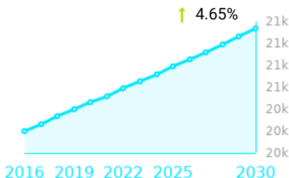
Population Growth
